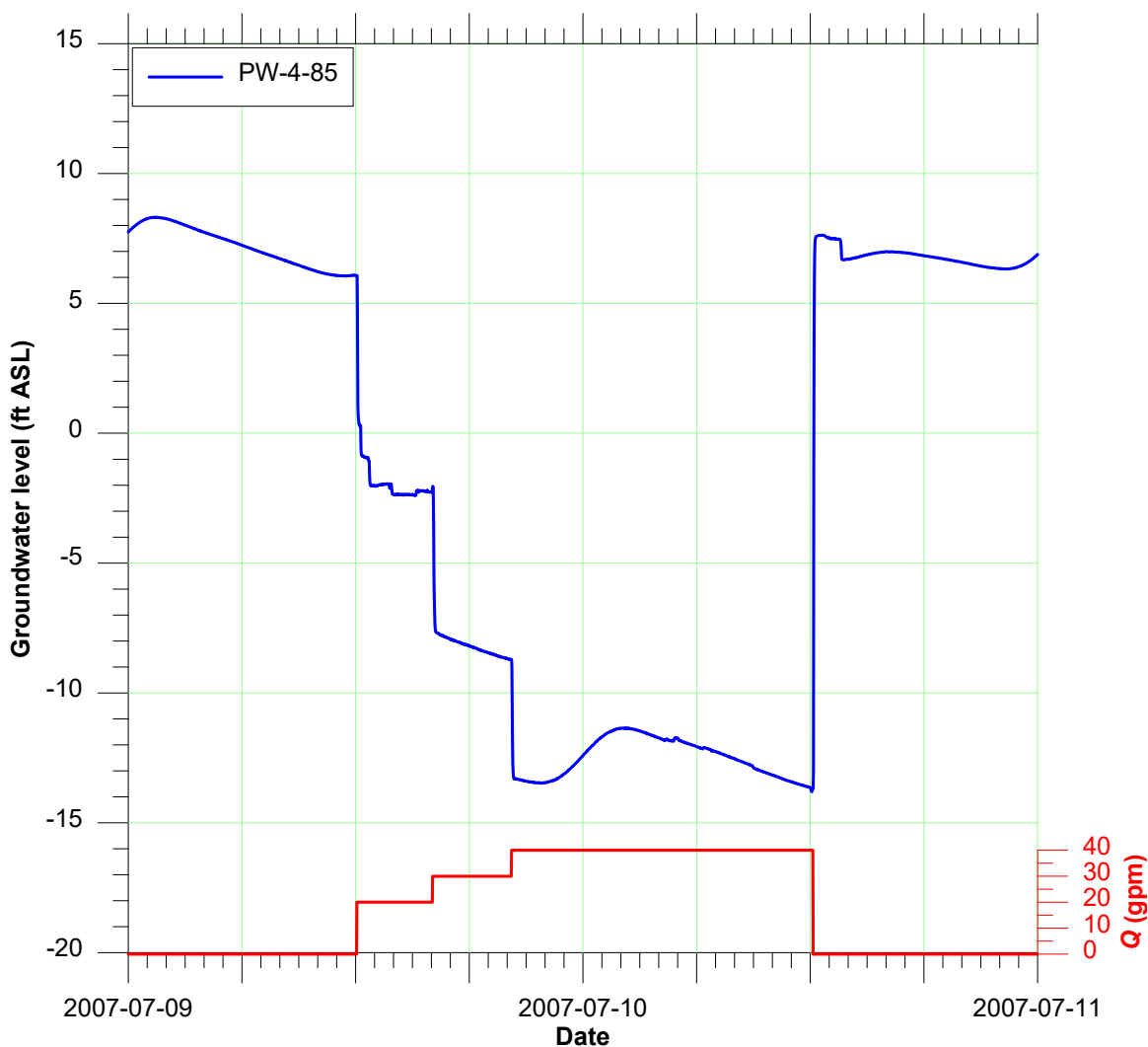
Figure 1. Data collected during a pumping test
