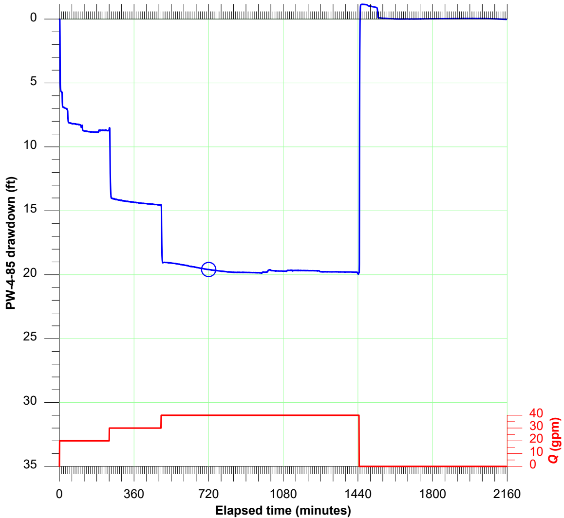
Figure 3. Interpreted drawdowns
