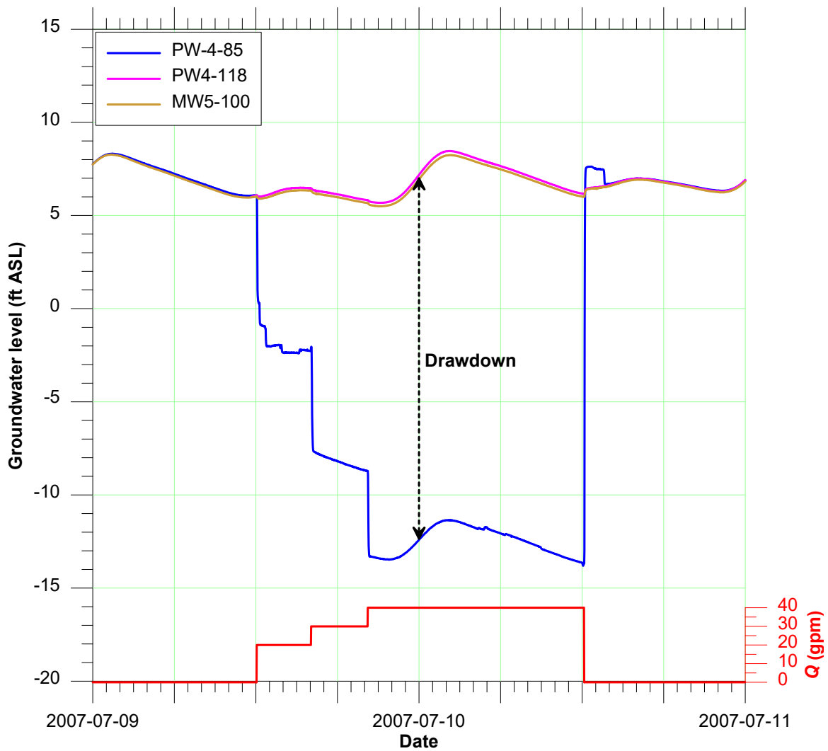
Figure 2. Water level records for the pumping well and adjacent observation wells
