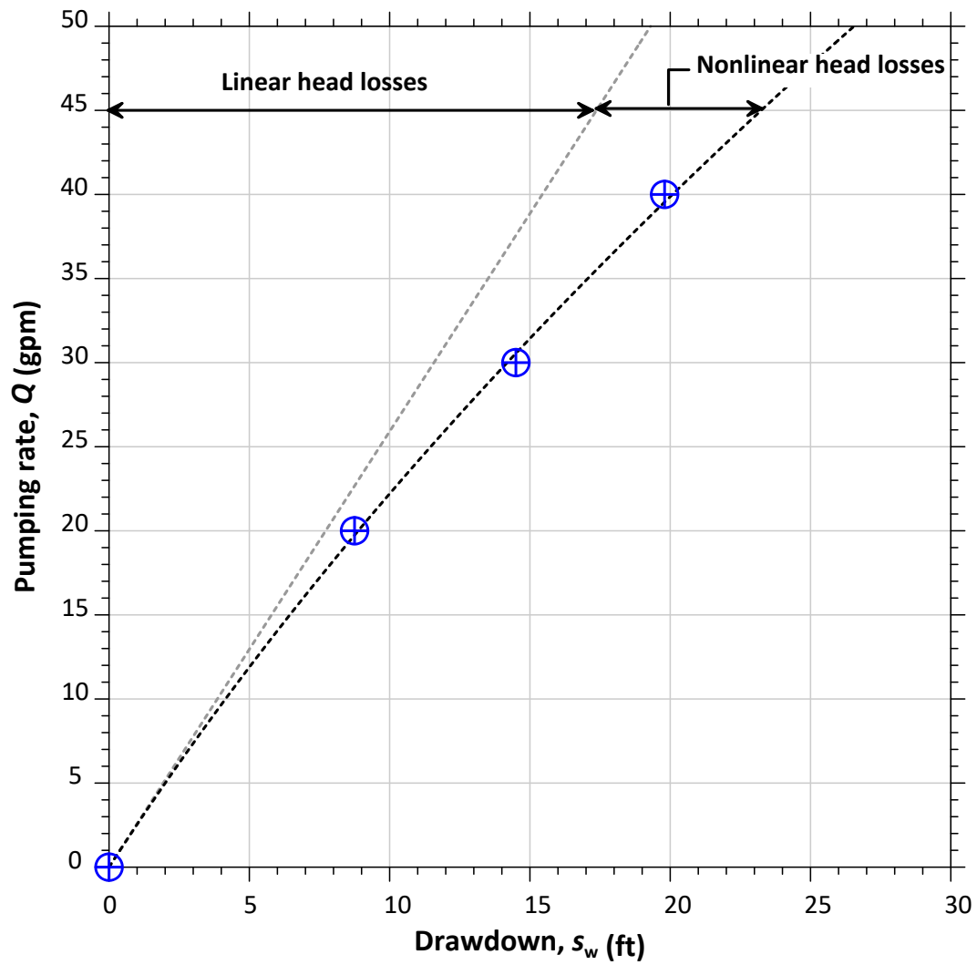
Figure 6. Identification of linear and nonlinear components of PW-4-85 drawdown
