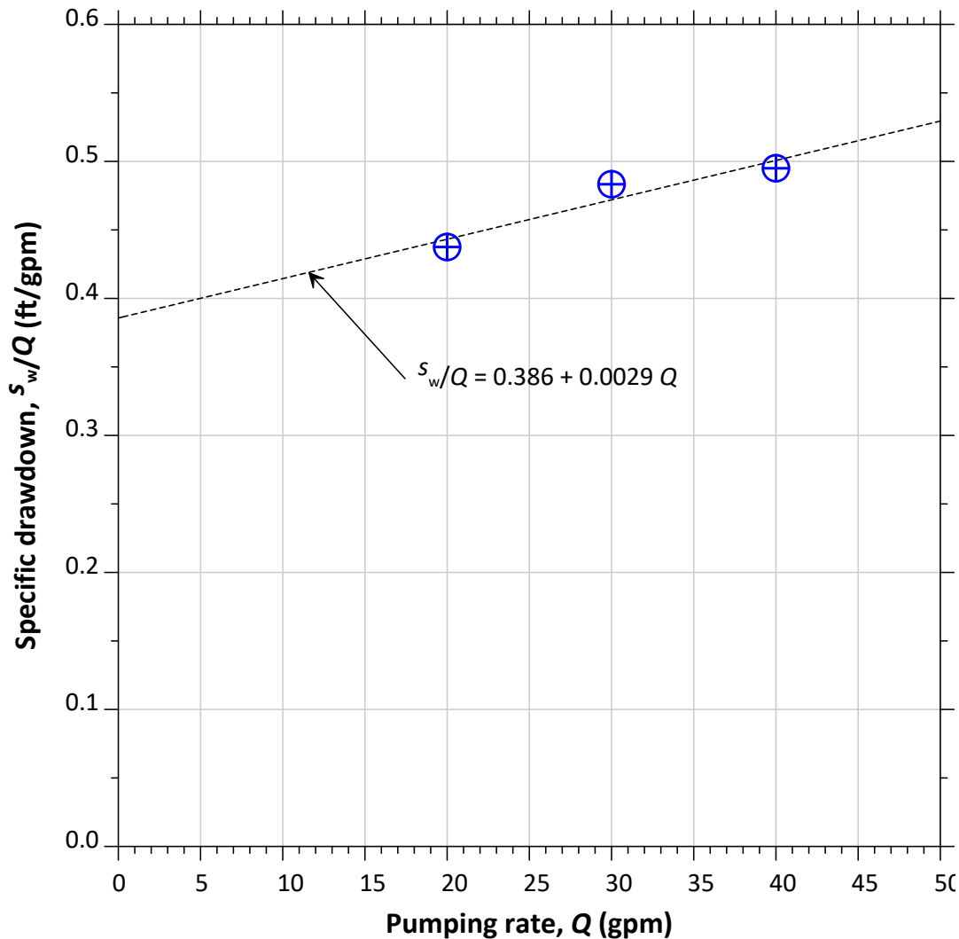
Figure 5. Hantush-Bierschenk analysis of PW-4-85 drawdowns
