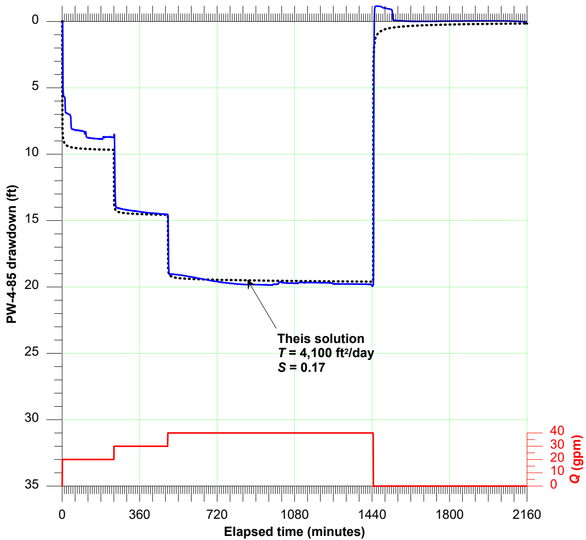
Figure 4. Match to the drawdowns with the Theis solution
