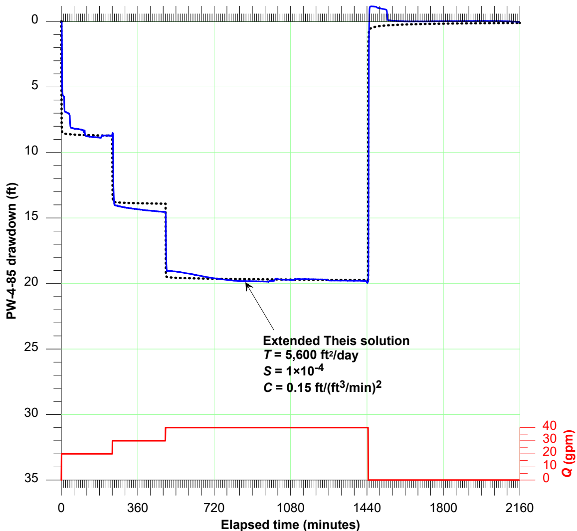
Figure 7. Alternative match to the drawdowns with the extended Theis solution
